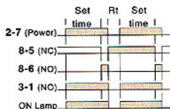
CONNECTION DIAGRAM
