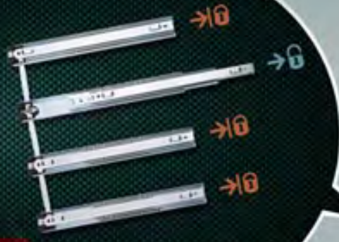
H57mm Interlock slide (Anti-tilt system)
